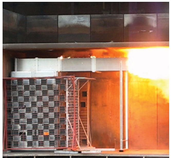
Internal arc fault test, 31.5kA/1s
